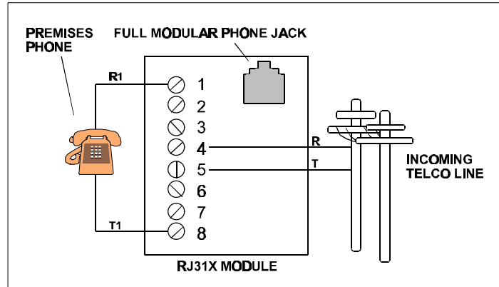
Figure 6: RJ31X Wiring
