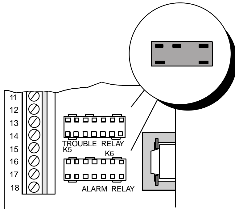
Figure 5: Relay Sockets
