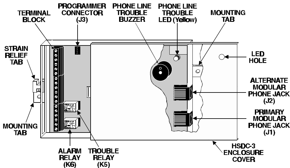
Figure 1: HSDC-3 Control/Communicator
