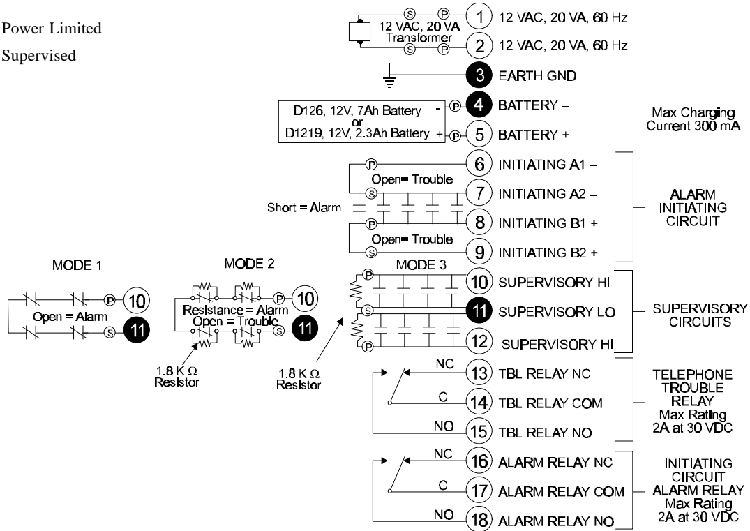
Figure 2: Stand-Alone Installation
