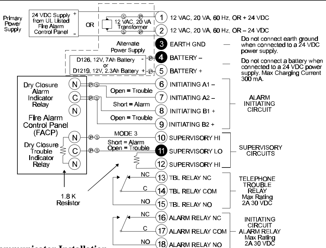
Figure 3: Slave Communicator Installation
